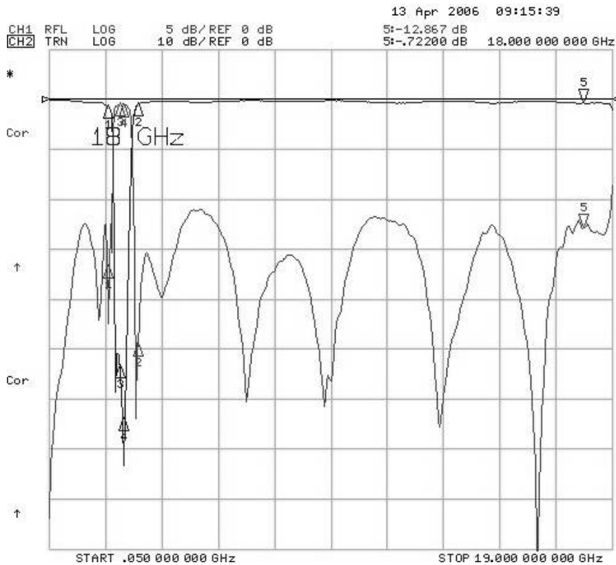
TYPICAL PERFORMANCE DATA FOR BRM50702
