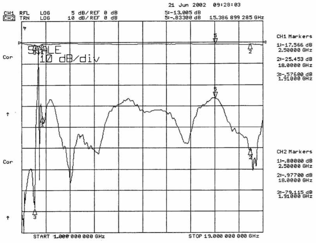
HPM50110 Typical Performance Data
